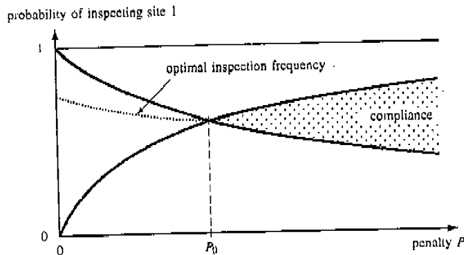
Fig. 1. Optimal inspection frequency for site 1 in the game of Table 2, versus punishment parameter P . Along each bold line, the inspectee is indifferent between violating and complying at one site. All violation is detected in the dotted area (where P > P_0 )
